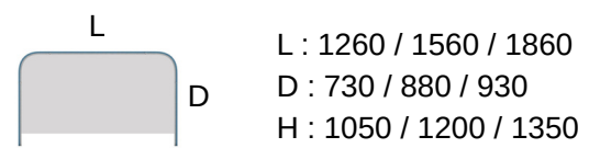
Reception Counter - Curved corners
